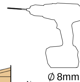
③ Windboard Assembly 3
