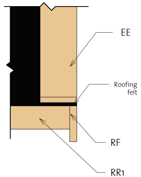
3 Roof Reinforcement
